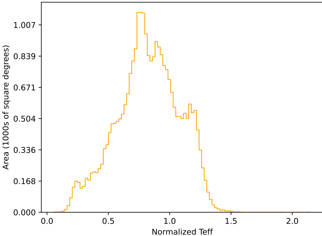
noroll_mjdp180_v3.4_10yrs All sky r band: Normalized Teff
