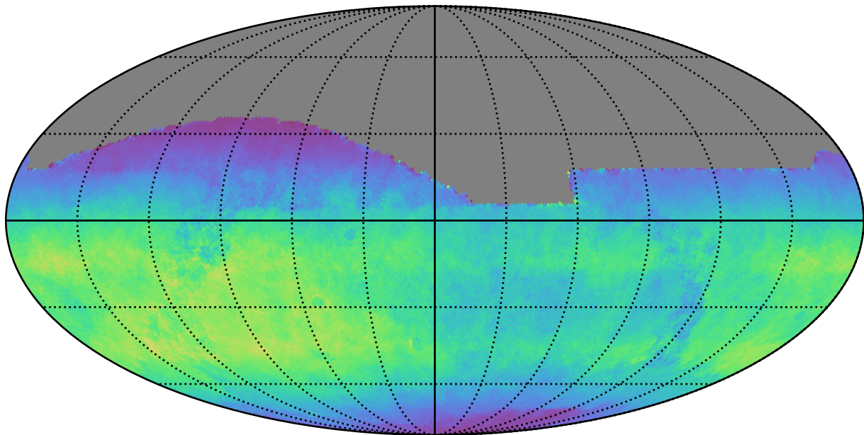
noroll_mjdp180_v3.4_10yrs All sky i band: Normalized Teff
