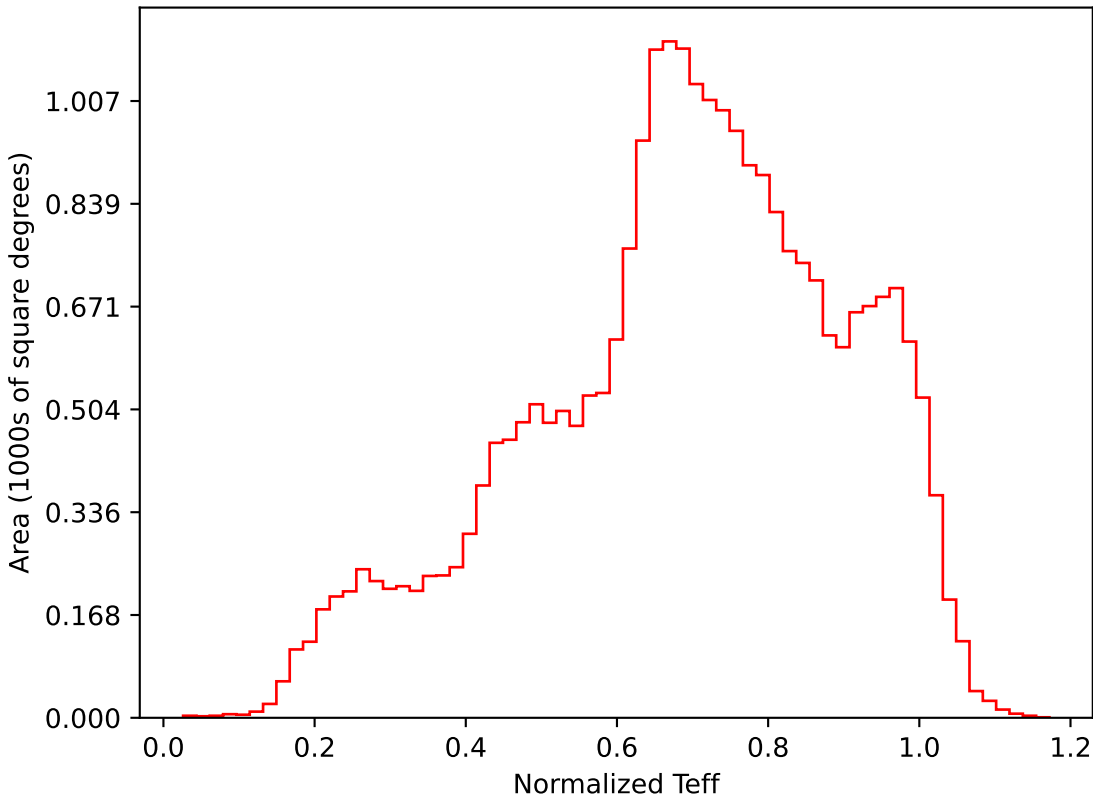
noroll_mjdp180_v3.4_10yrs All sky i band: Normalized Teff
