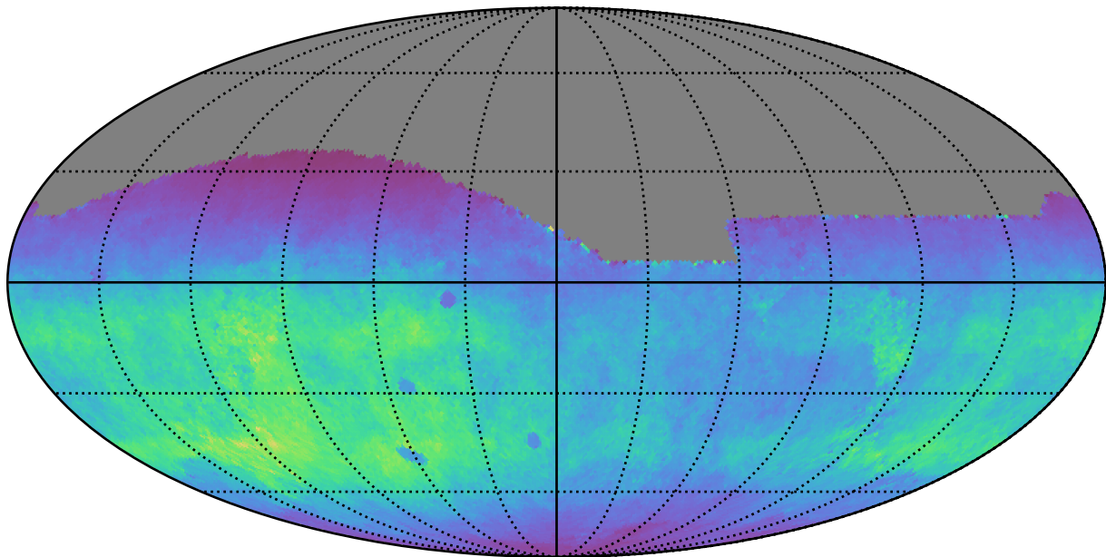
noroll_mjdp180_v3.4_10yrs All sky g band: Normalized Teff
