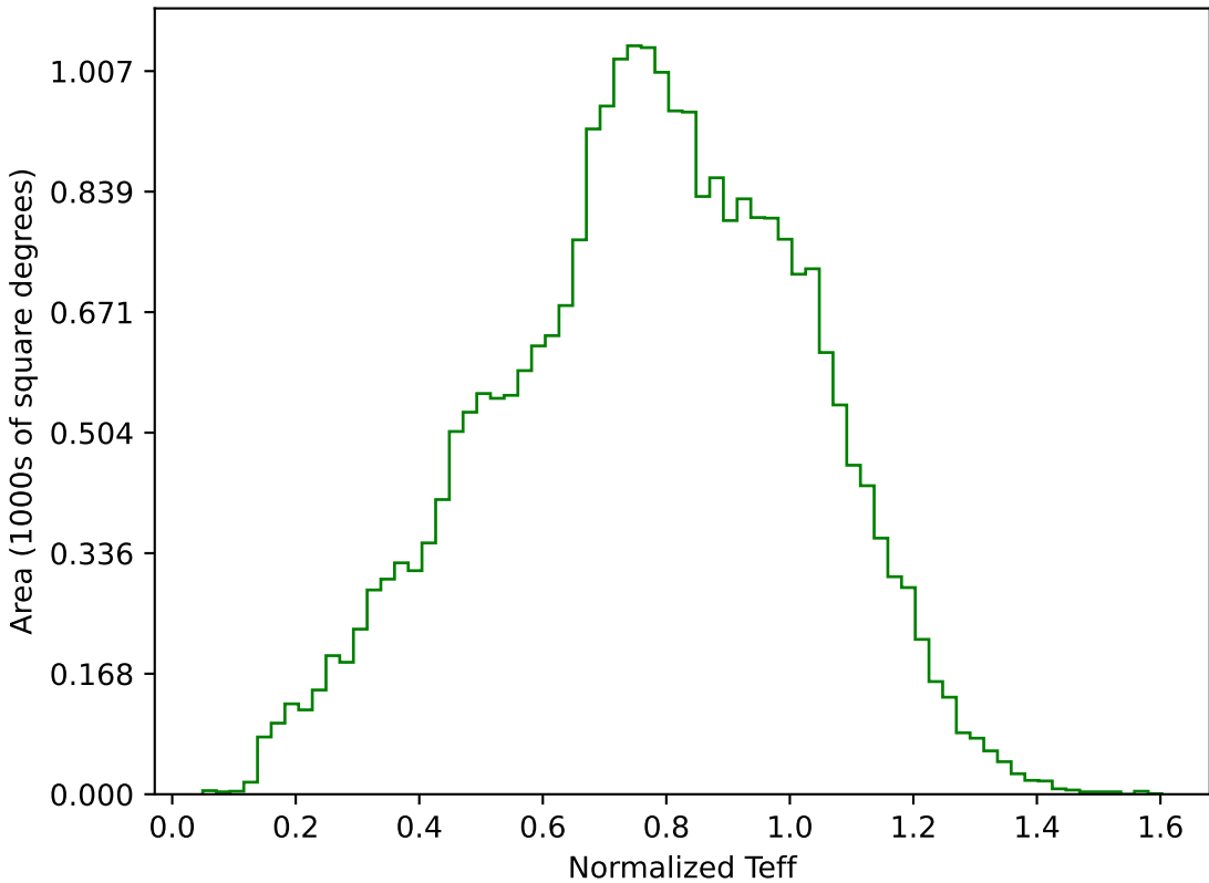
noroll_mjdp180_v3.4_10yrs All sky g band: Normalized Teff
