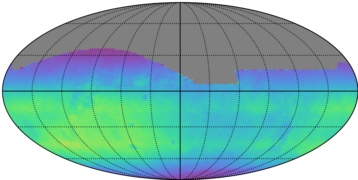
noroll_mjdp180_v3.4_10yrs All sky all bands: Normalized Teff
