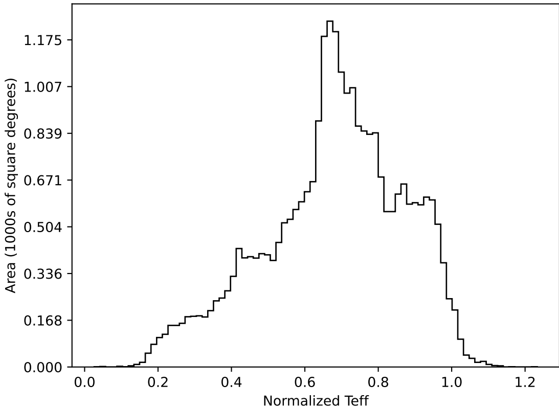
noroll_mjdp180_v3.4_10yrs All sky all bands: Normalized Teff
