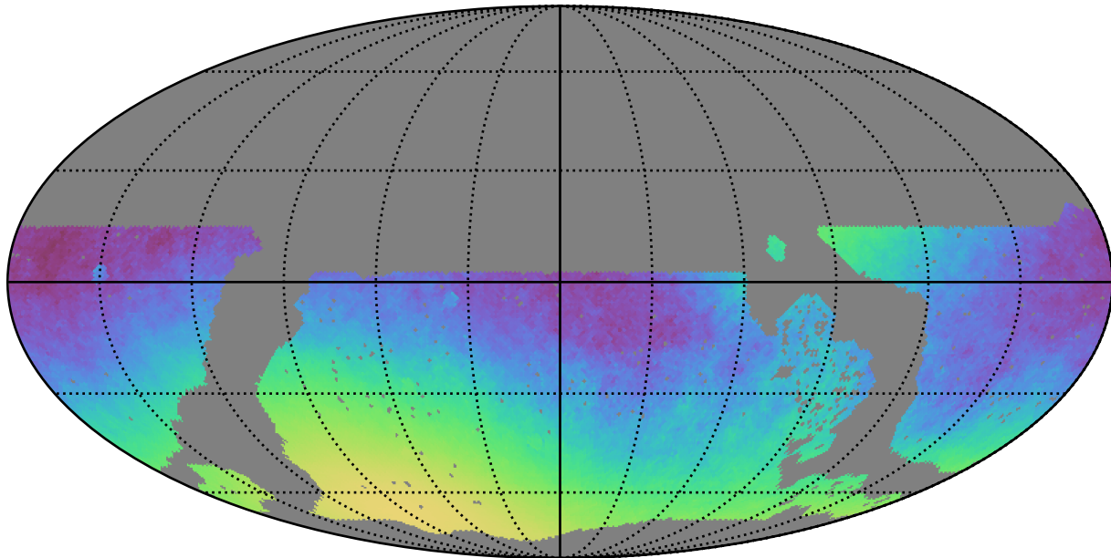
noroll_mjdp180_v3.4_10yrs WFD: Normalized Parallax Uncert @ 24.0
