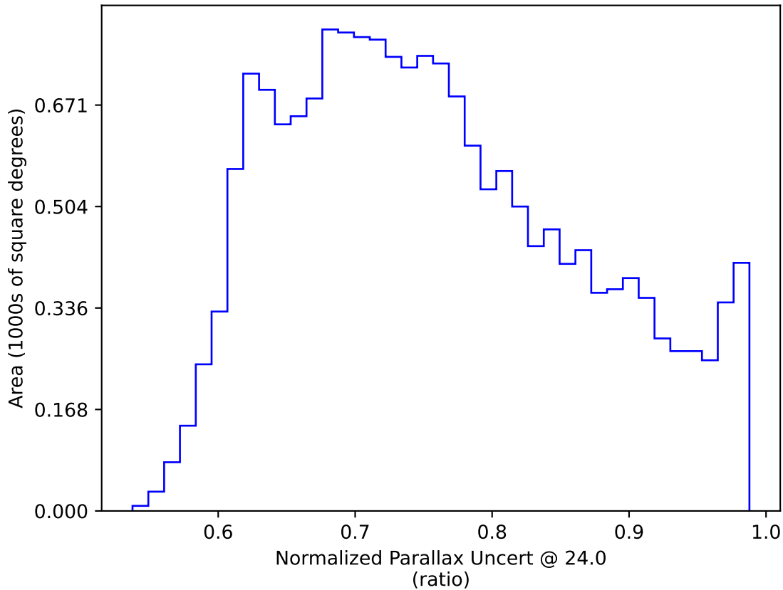
noroll_mjdp180_v3.4_10yrs WFD: Normalized Parallax Uncert @ 24.0
