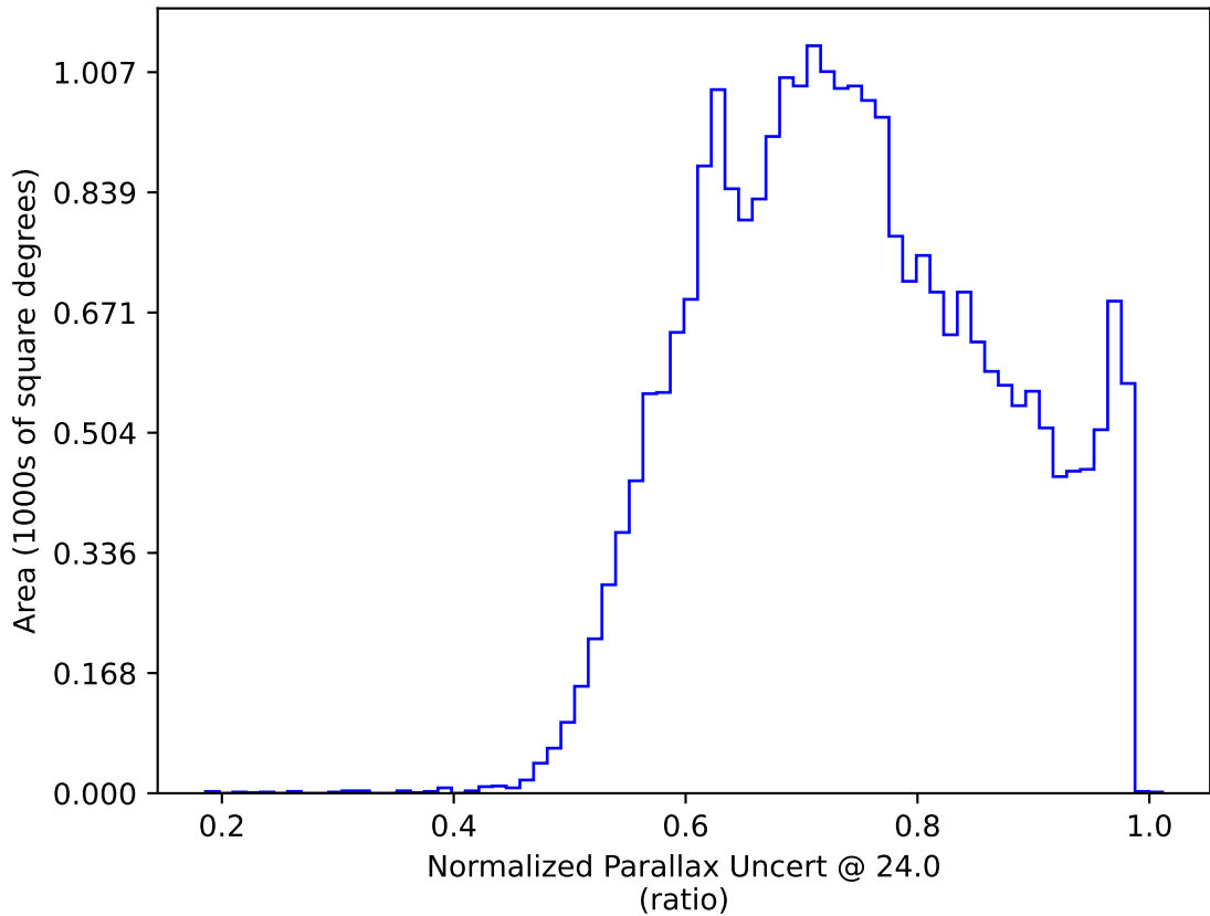
noroll_mjdp180_v3.4_10yrs All sky: Normalized Parallax Uncert @ 24.0
