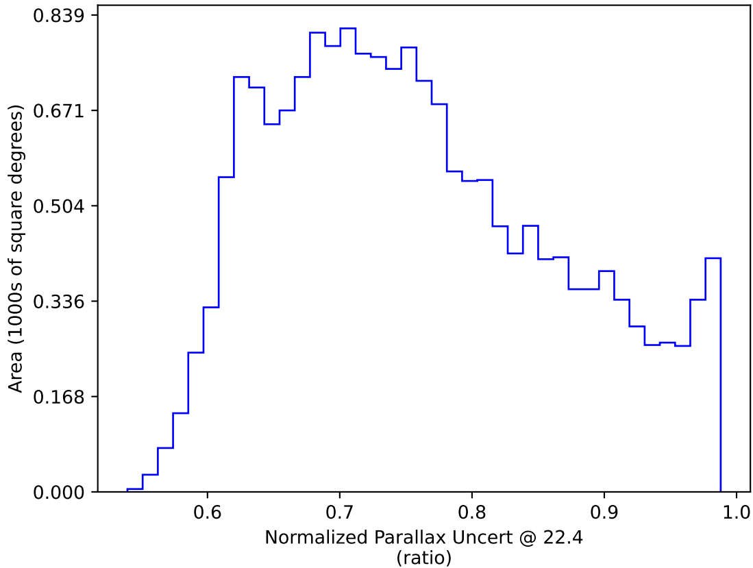
noroll_mjdp180_v3.4_10yrs WFD: Normalized Parallax Uncert @ 22.4
