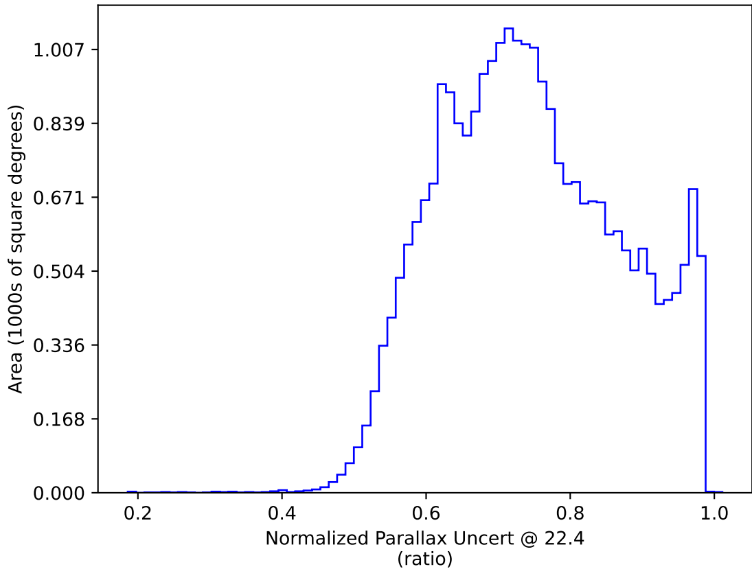
noroll_mjdp180_v3.4_10yrs All sky: Normalized Parallax Uncert @ 22.4
