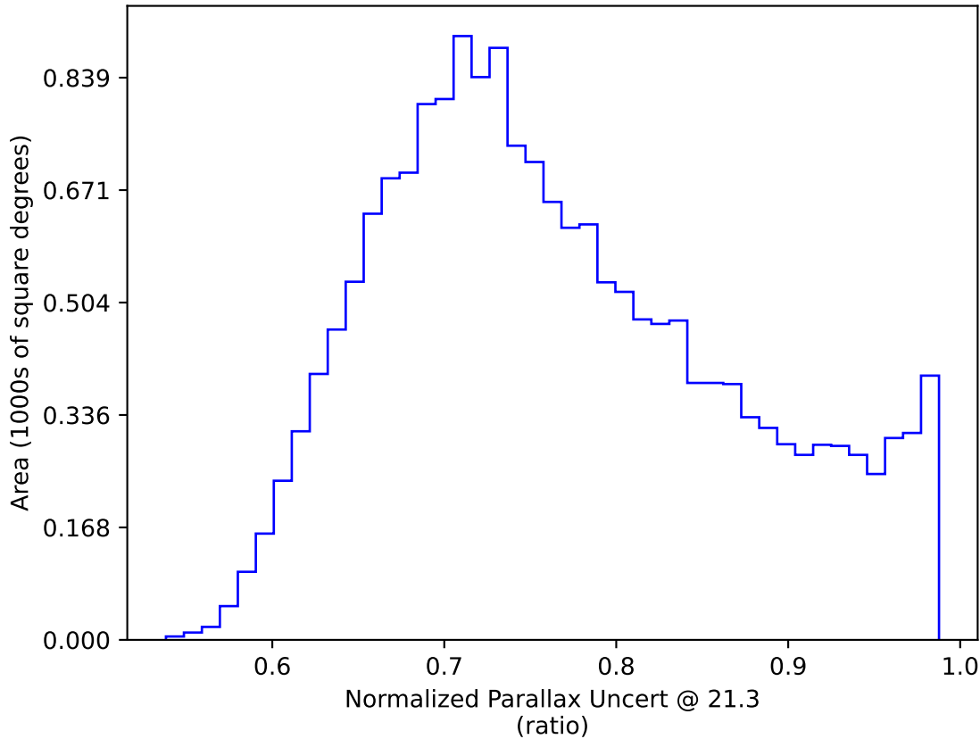
noroll_mjdp180_v3.4_10yrs WFD y band only: Normalized Parallax Uncert @ 21.3
