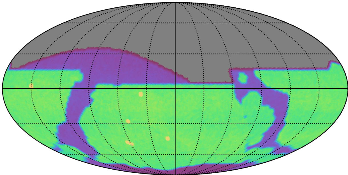
noroll_mjdp180_v3.4_10yrs All sky all bands: N Unique Nights
