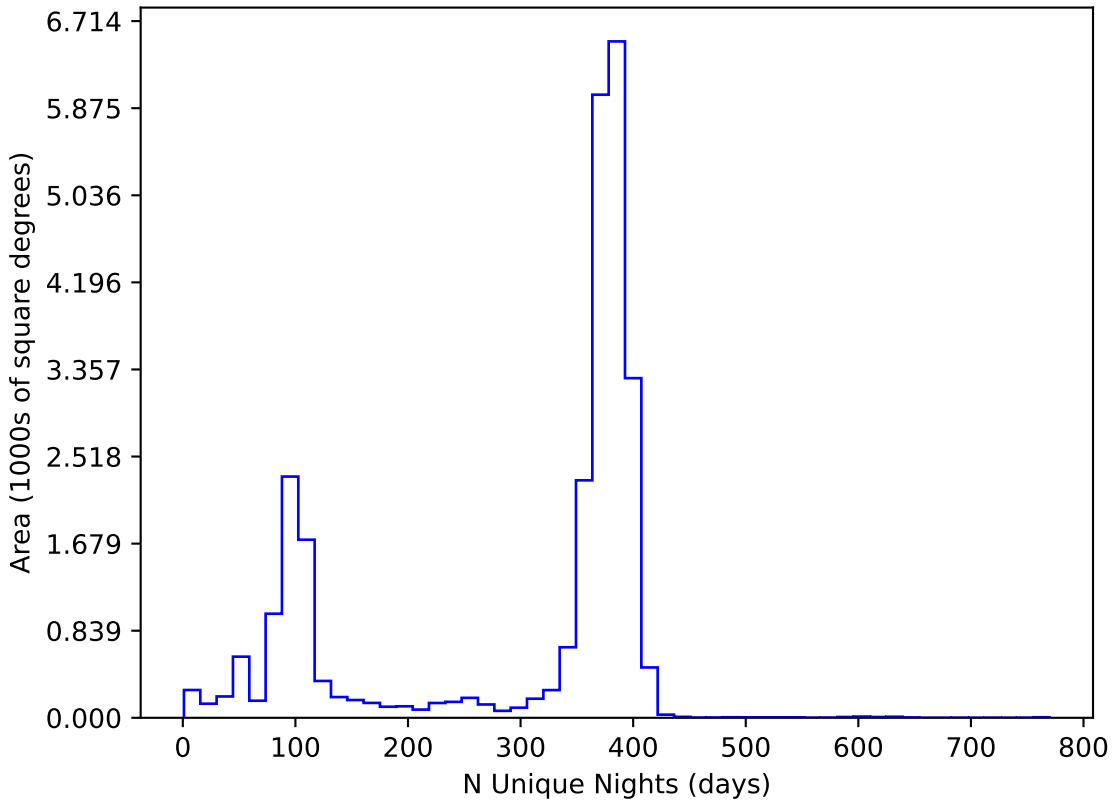
noroll_mjdp180_v3.4_10yrs All sky all bands: N Unique Nights
