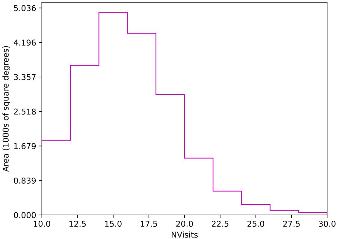
noroll_mjdp180_v3.4_10yrs Yr 3-4 z band: NVisits
