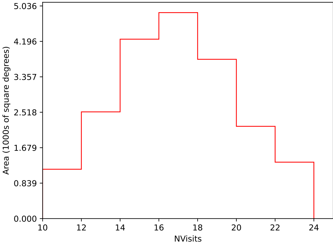
noroll_mjdp180_v3.4_10yrs Yr 3-4 i band: NVisits
