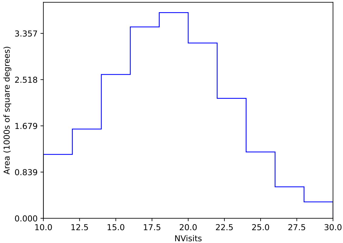
noroll_mjdp180_v3.4_10yrs Yr 1 y band: NVisits
