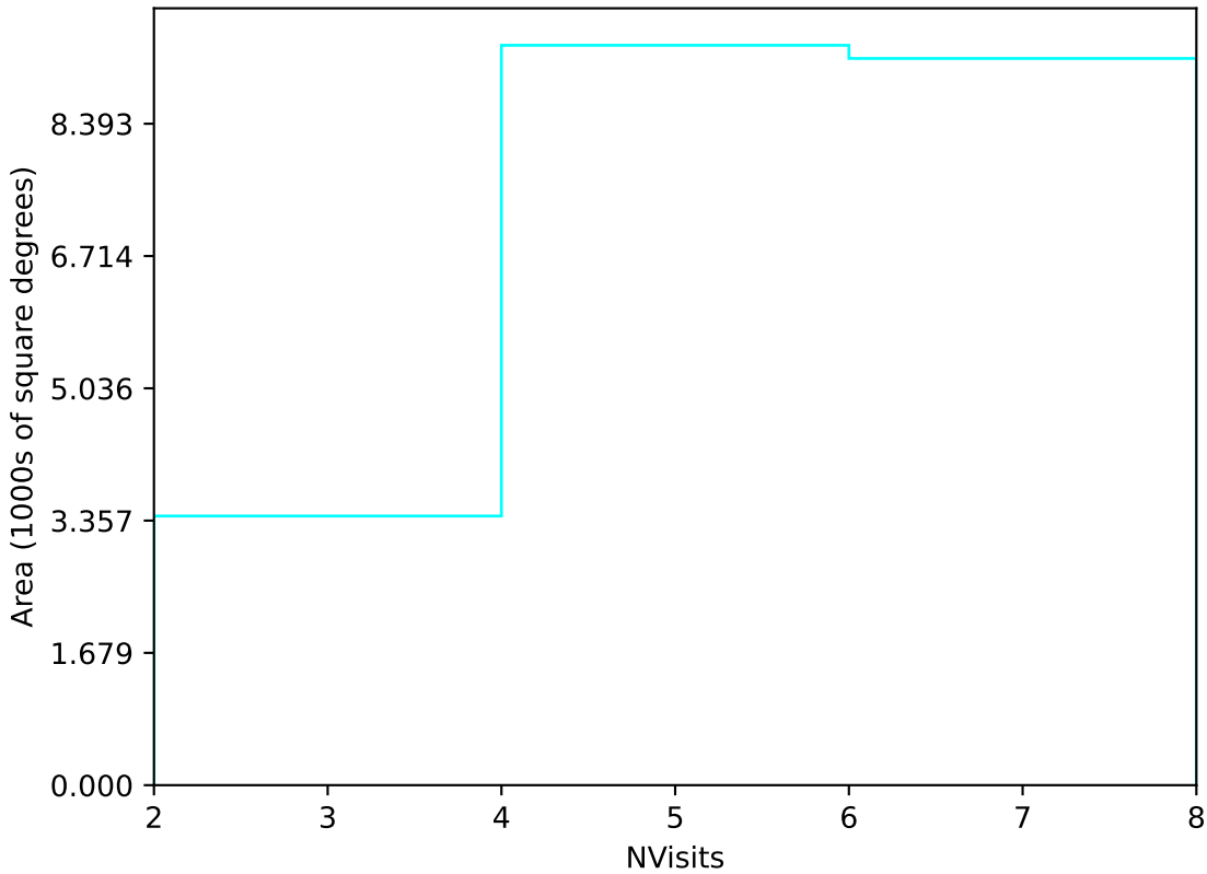
noroll_mjdp180_v3.4_10yrs Yr 1 u band: NVisits
