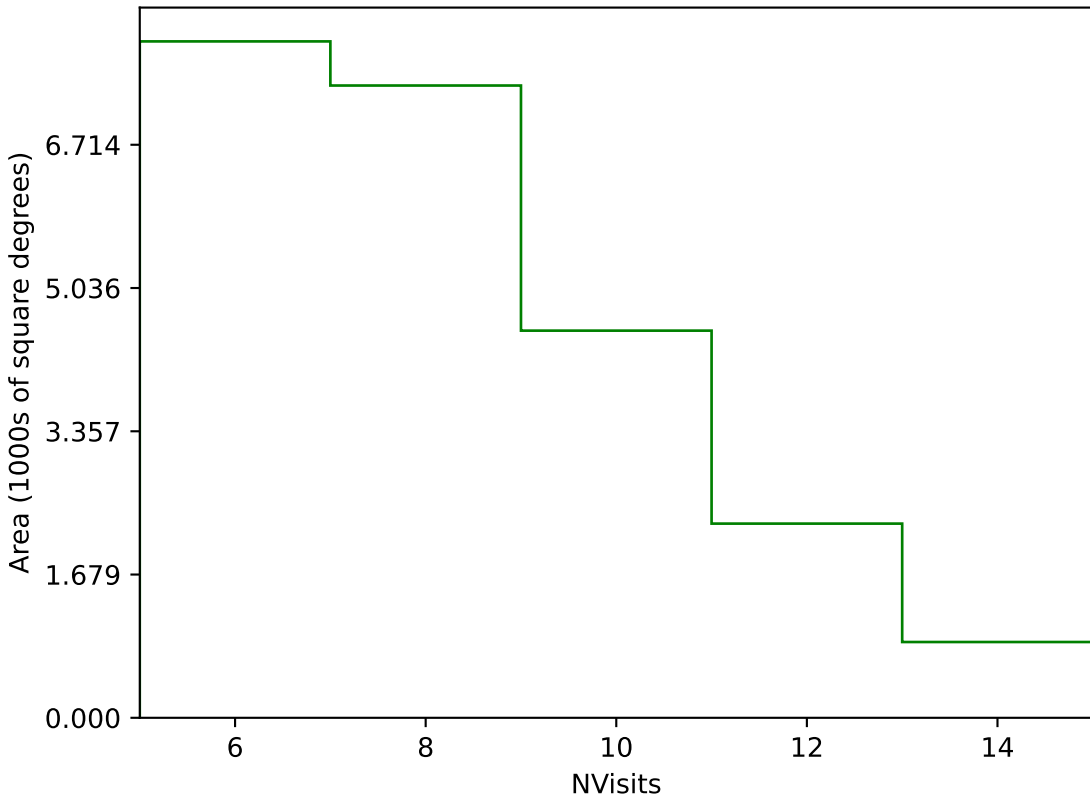
noroll_mjdp180_v3.4_10yrs Yr 1 g band: NVisits
