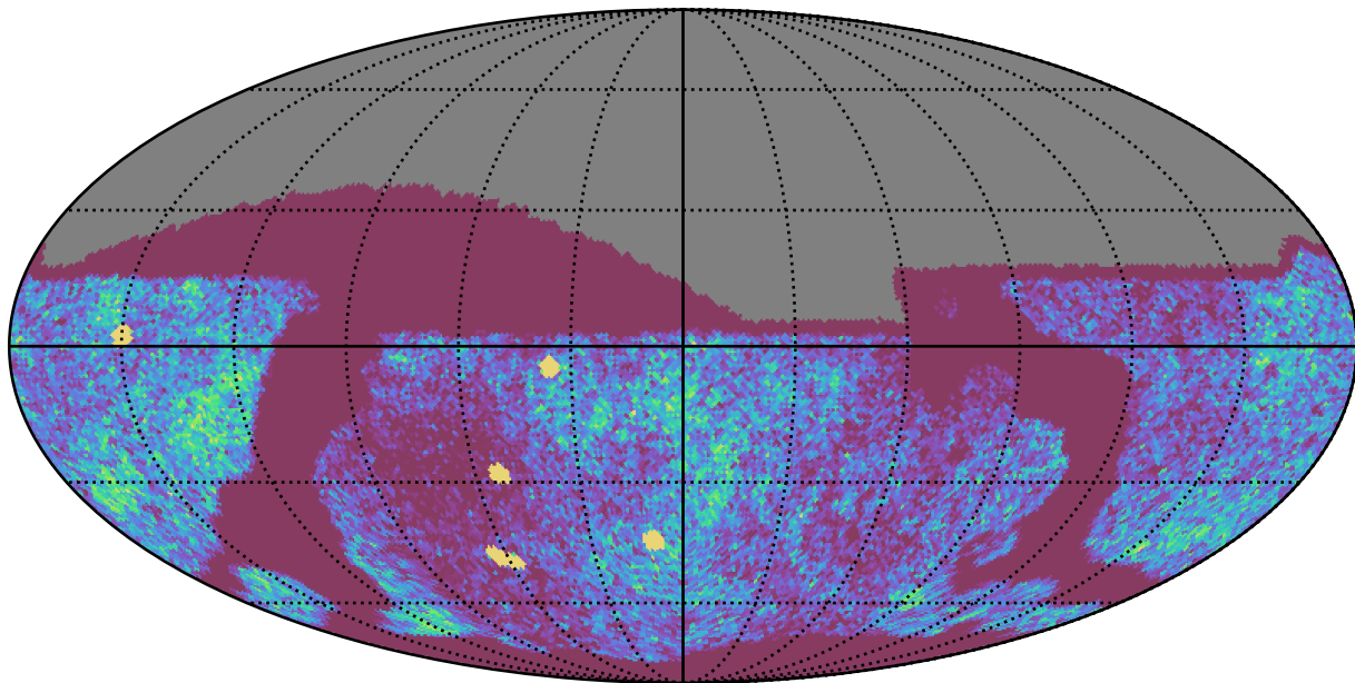
noroll_mjdp180_v3.4_10yrs Yr 1 all bands: NVisits
