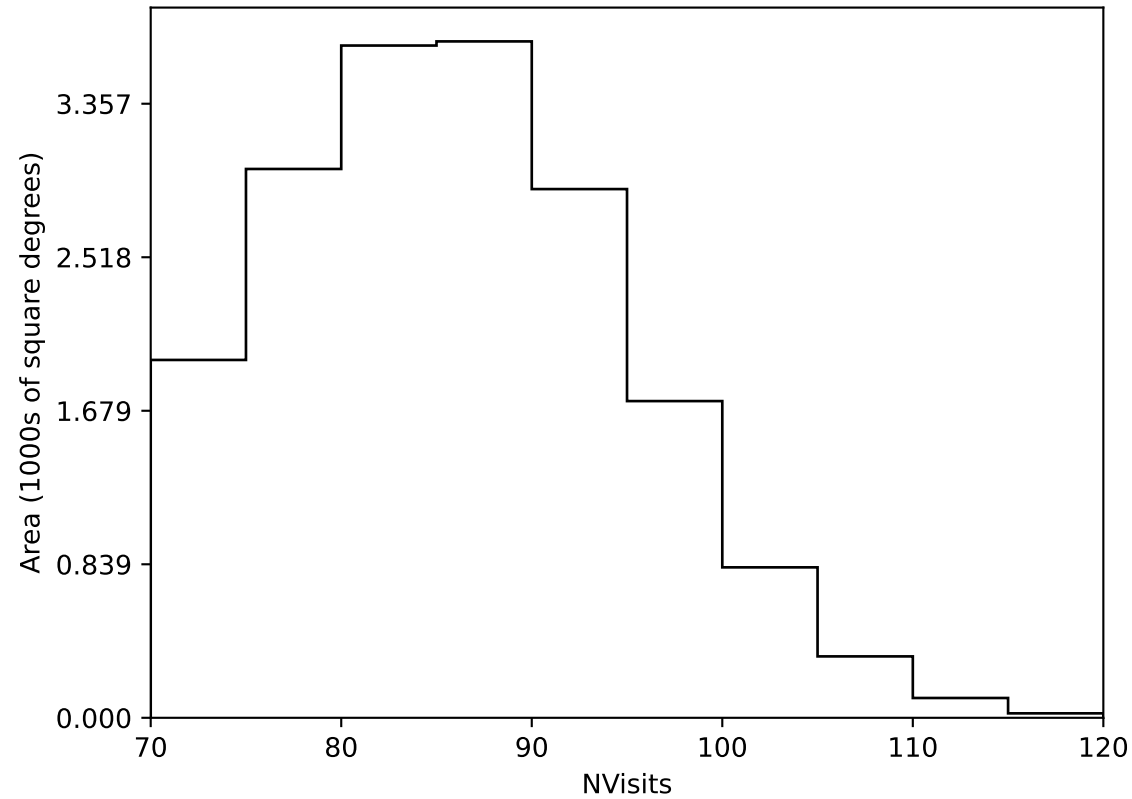
noroll_mjdp180_v3.4_10yrs Yr 1 all bands: NVisits
