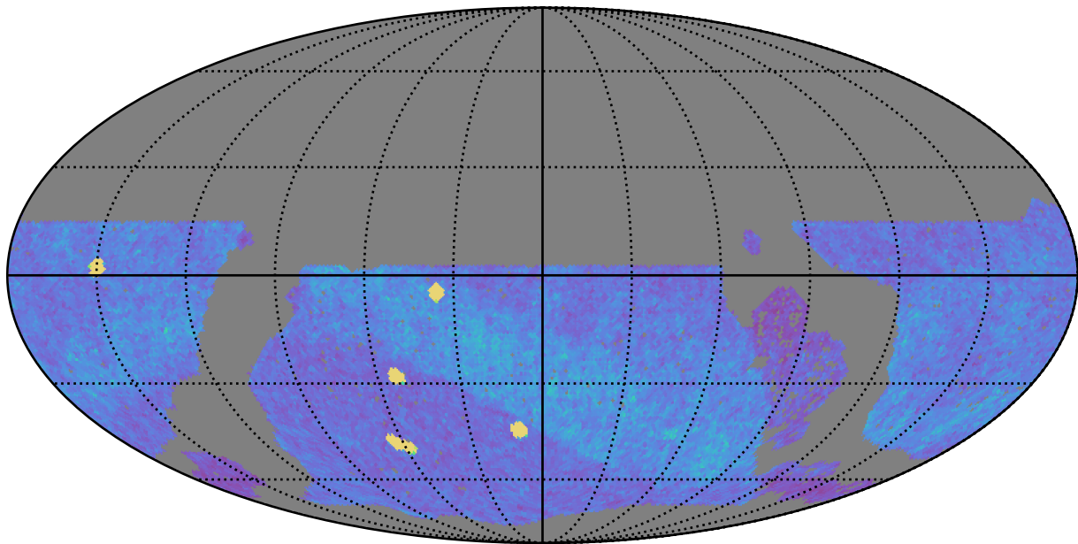
noroll_mjdp180_v3.4_10yrs WFD z band: NVisits
