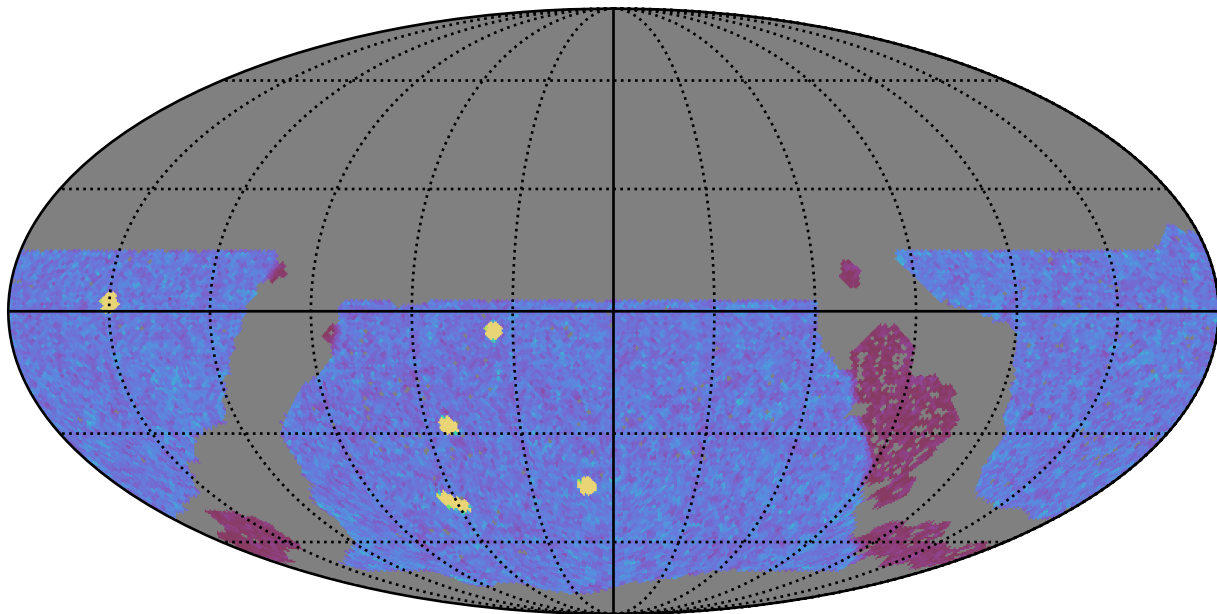
noroll_mjdp180_v3.4_10yrs WFD y band: NVisits
