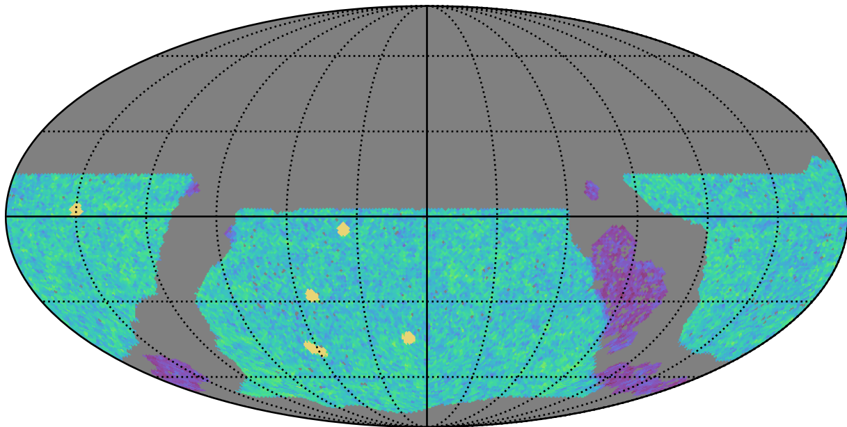
noroll_mjdp180_v3.4_10yrs WFD u band: NVisits
