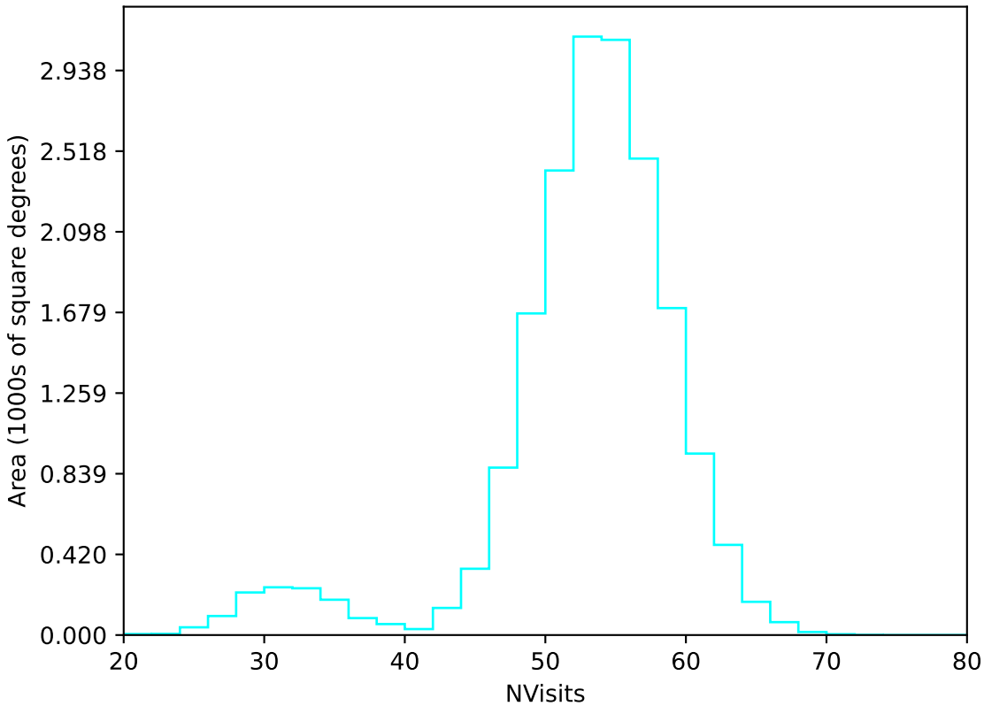
noroll_mjdp180_v3.4_10yrs WFD u band: NVisits
