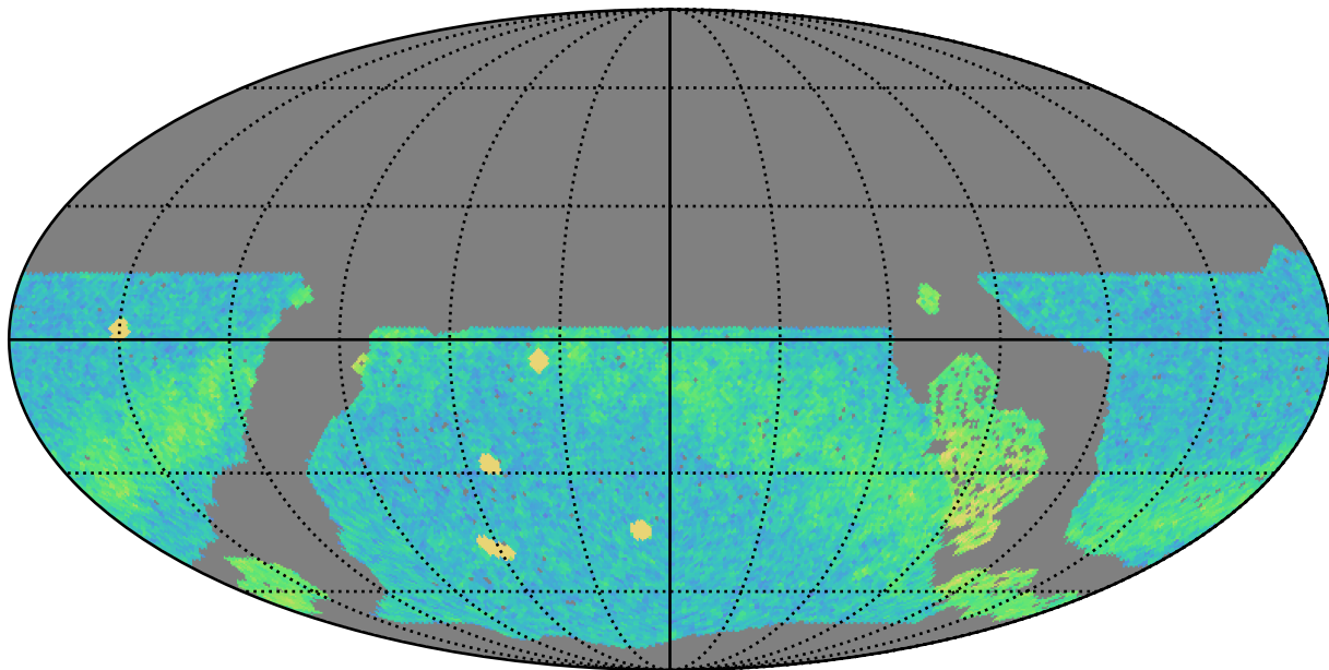
noroll_mjdp180_v3.4_10yrs WFD r band: NVisits
