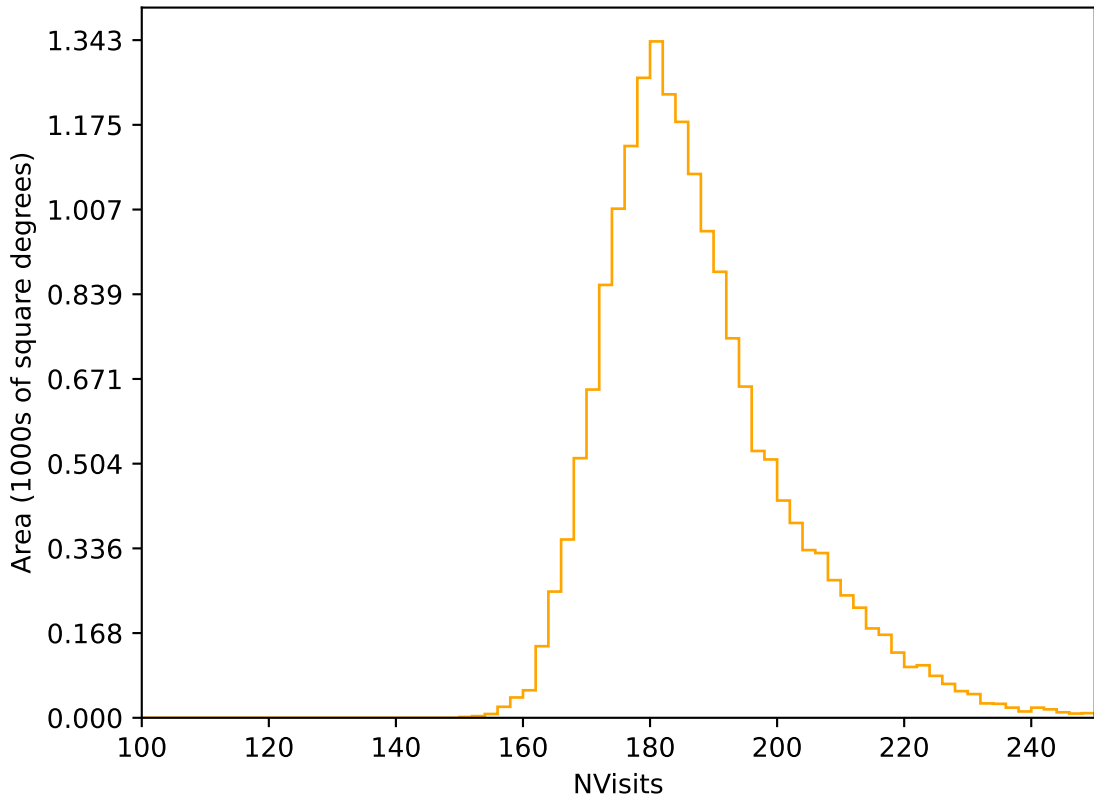
noroll_mjdp180_v3.4_10yrs WFD r band: NVisits
