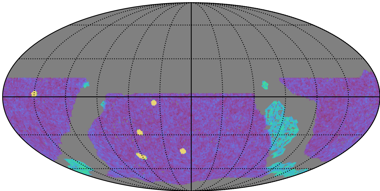
noroll_mjdp180_v3.4_10yrs WFD g band: NVisits
