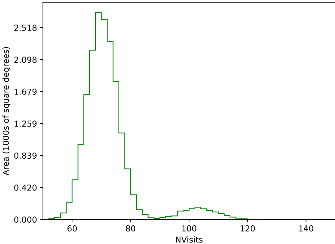
noroll_mjdp180_v3.4_10yrs WFD g band: NVisits
