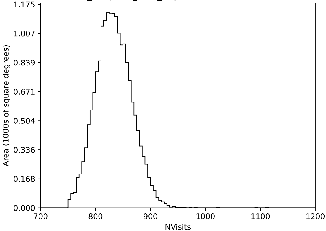
noroll_mjdp180_v3.4_10yrs WFD all bands: NVisits
