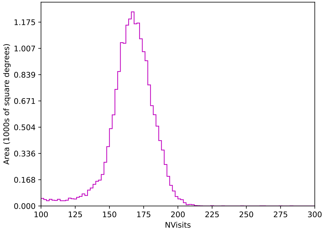
noroll_mjdp180_v3.4_10yrs All sky z band: NVisits
