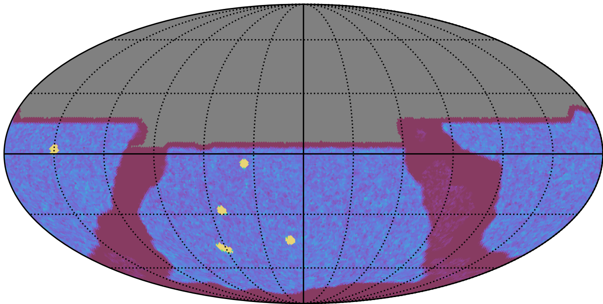
noroll_mjdp180_v3.4_10yrs All sky y band: NVisits
