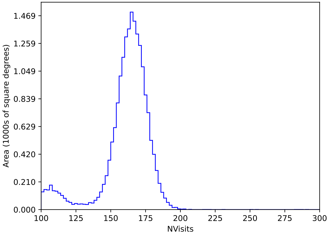
noroll_mjdp180_v3.4_10yrs All sky y band: NVisits
