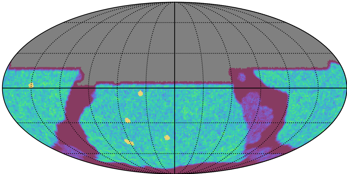
noroll_mjdp180_v3.4_10yrs All sky u band: NVisits
