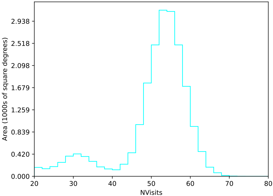
noroll_mjdp180_v3.4_10yrs All sky u band: NVisits
