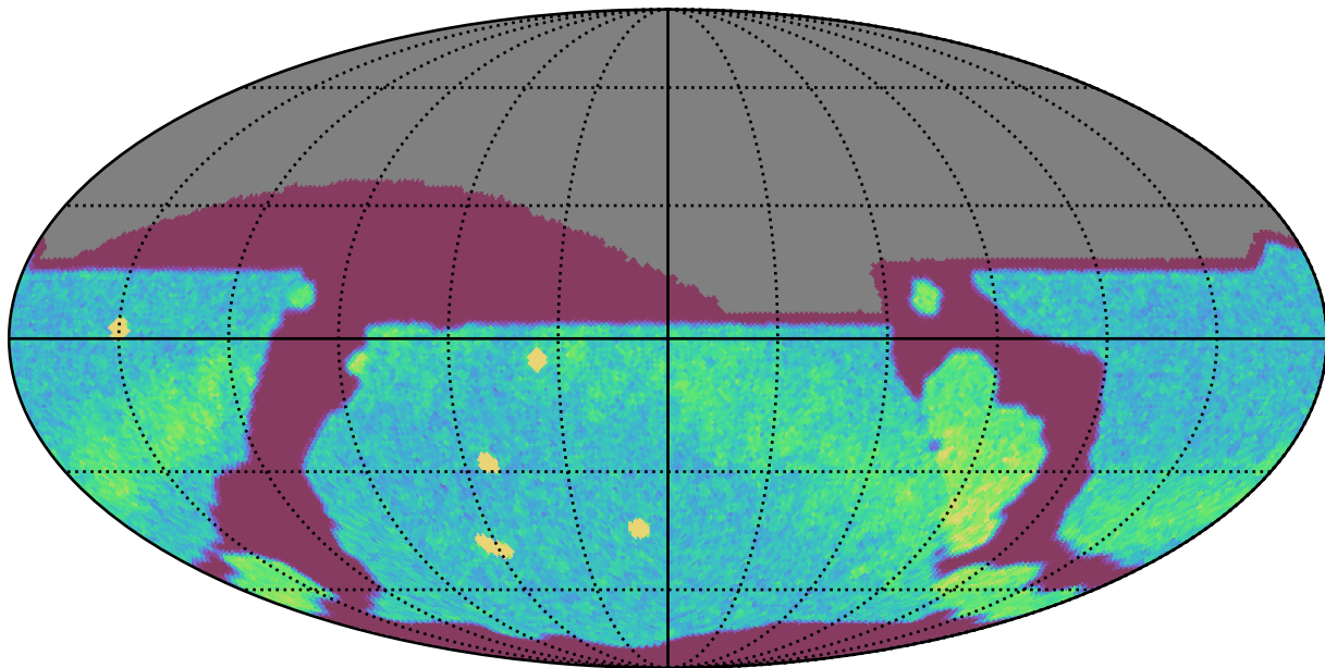
noroll_mjdp180_v3.4_10yrs All sky r band: NVisits
