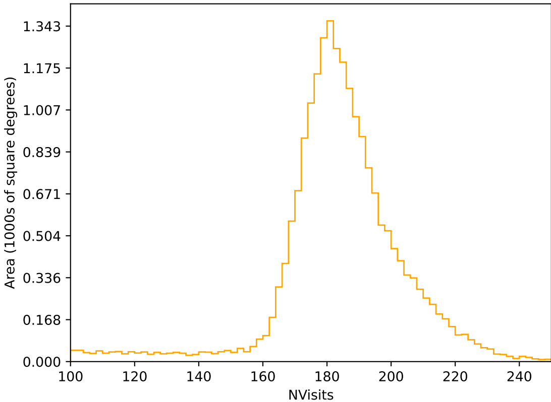
noroll_mjdp180_v3.4_10yrs All sky r band: NVisits
