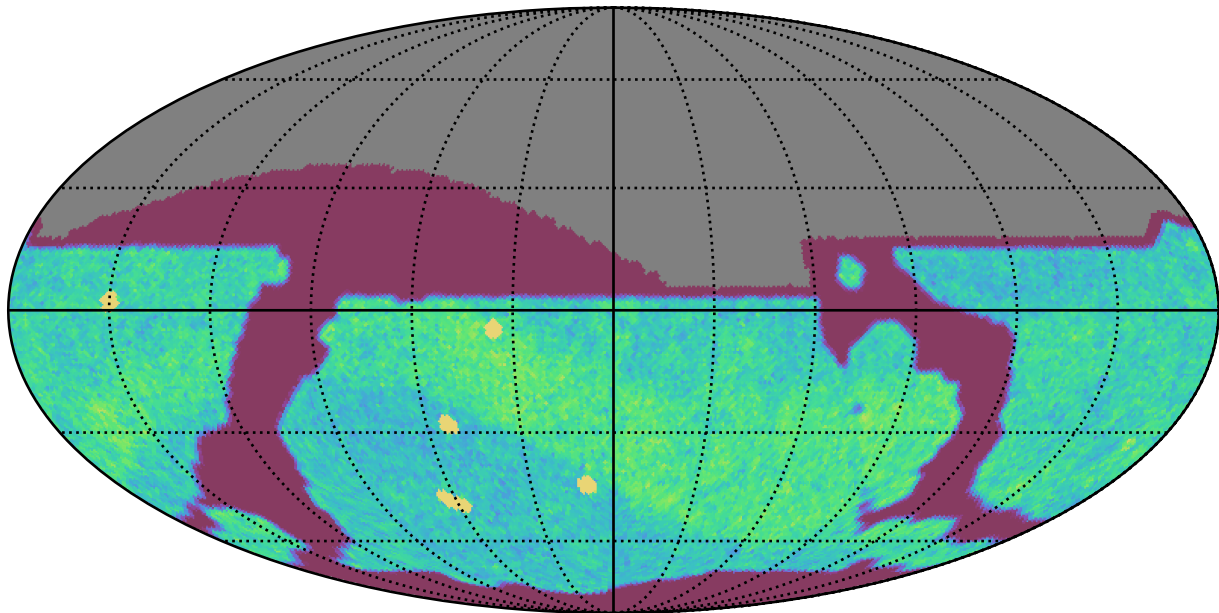
noroll_mjdp180_v3.4_10yrs All sky i band: NVisits
