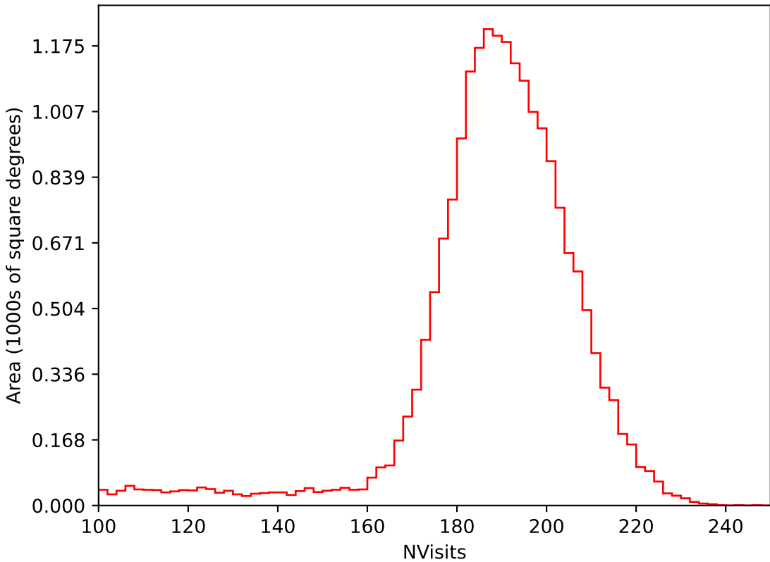
noroll_mjdp180_v3.4_10yrs All sky i band: NVisits
