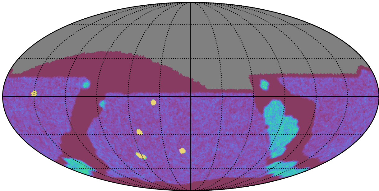
noroll_mjdp180_v3.4_10yrs All sky g band: NVisits
