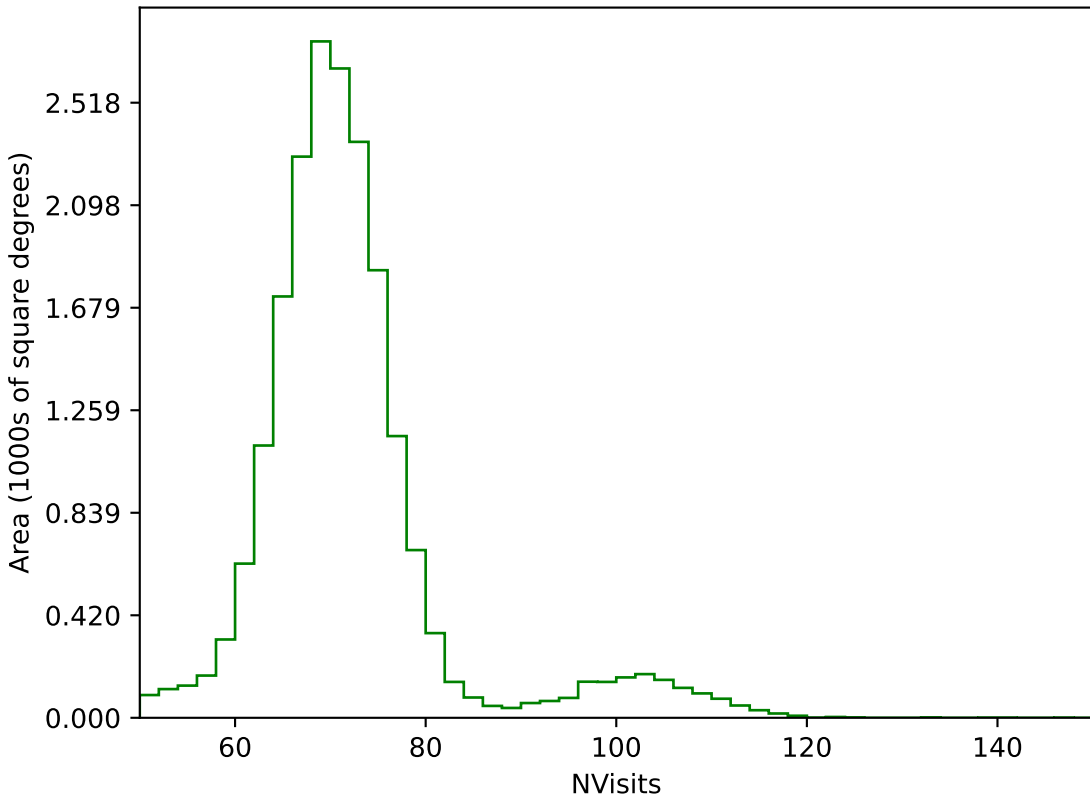
noroll_mjdp180_v3.4_10yrs All sky g band: NVisits
