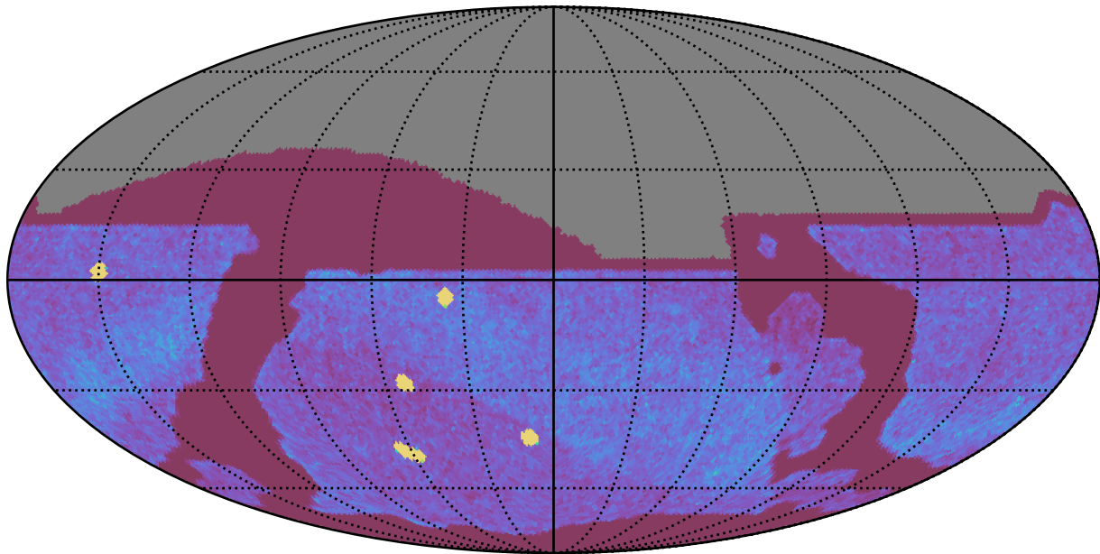
noroll_mjdp180_v3.4_10yrs All sky all bands: NVisits
