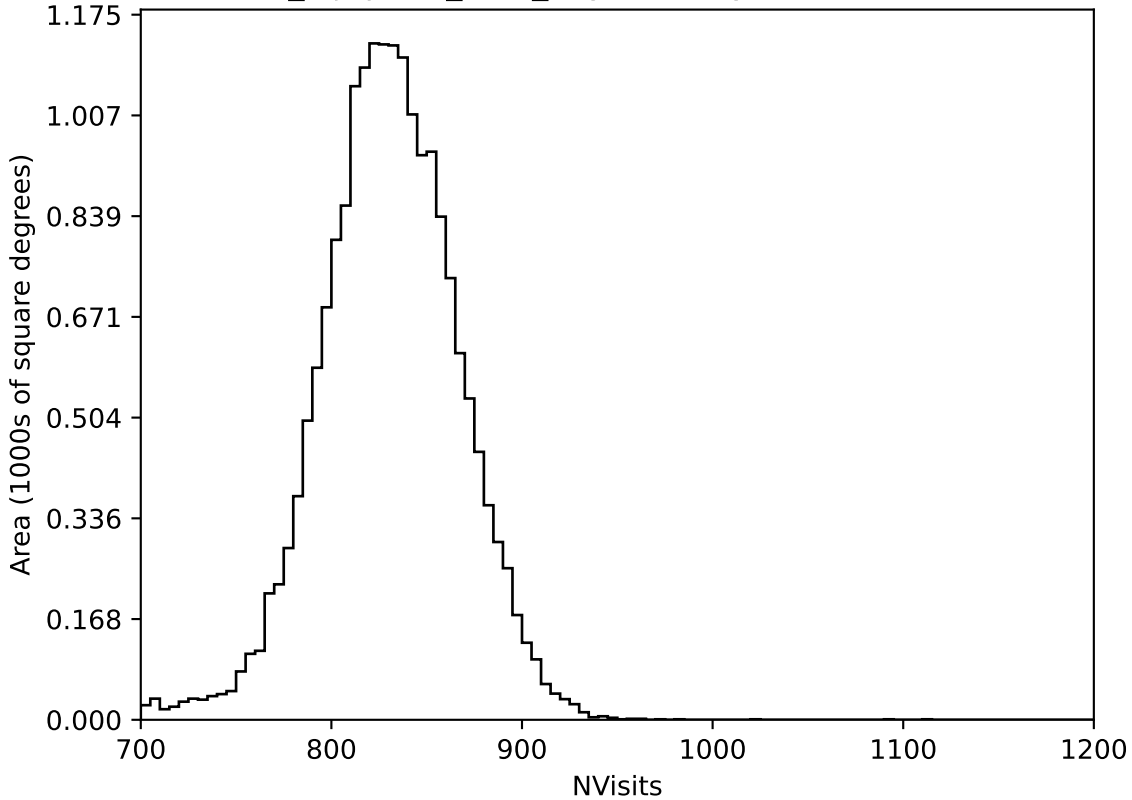
noroll_mjdp180_v3.4_10yrs All sky all bands: NVisits
