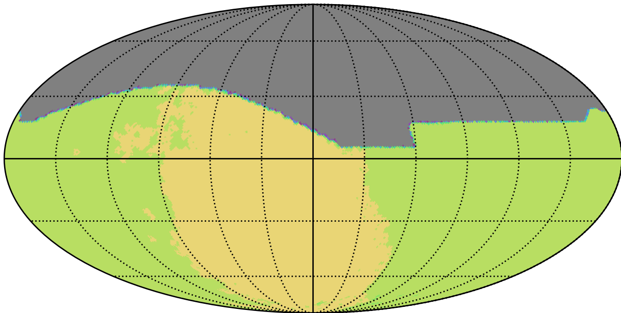
noroll_mjdp180_v3.4_10yrs All sky all bands: NSeasons
