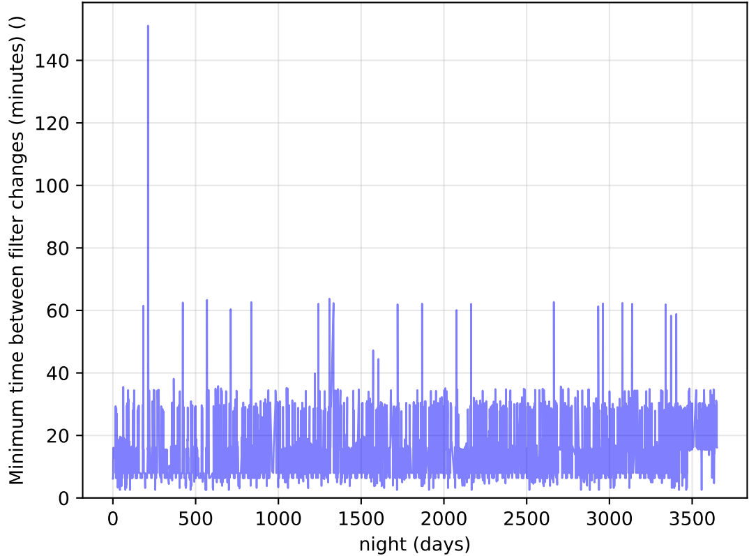
noroll_mjdp180_v3.4_10yrs Per Night: Minimum time between filter changes (minutes)
