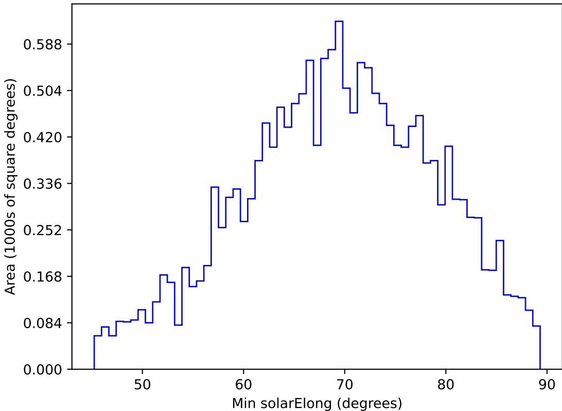
noroll_mjdp180_v3.4_10yrs WFD y band: Min solarElong
