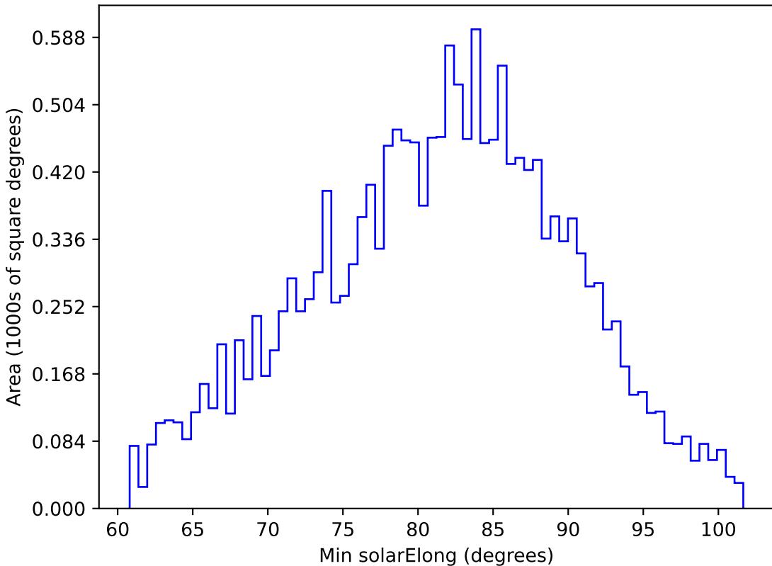
noroll_mjdp180_v3.4_10yrs WFD u band: Min solarElong
