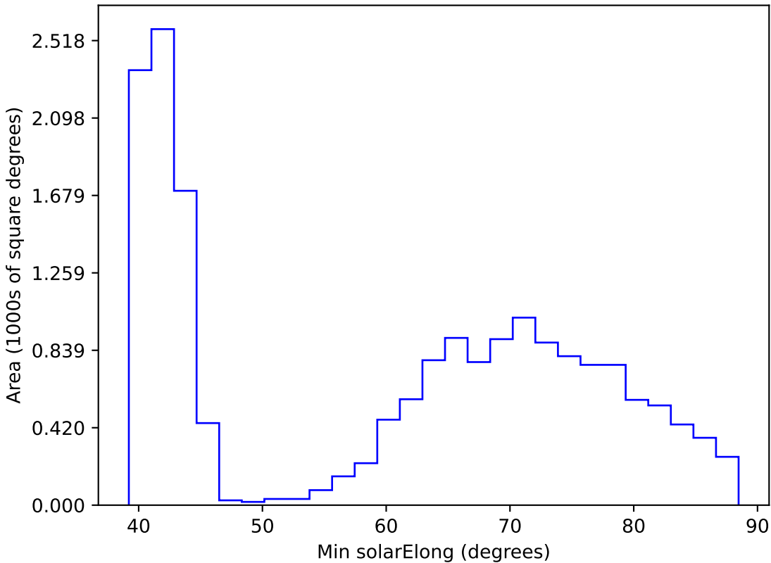
noroll_mjdp180_v3.4_10yrs WFD r band: Min solarElong
