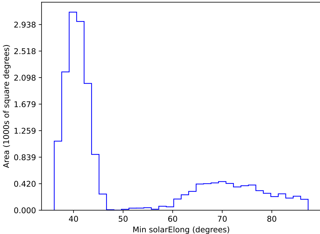
noroll_mjdp180_v3.4_10yrs WFD i band: Min solarElong
